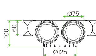
ceiling-mounted version
