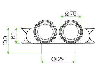
ceiling-mounted version
