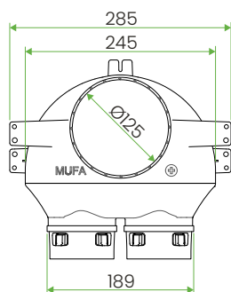
floor-mounted version
