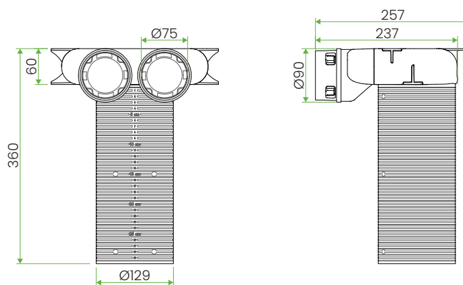
ceiling-mounted version
