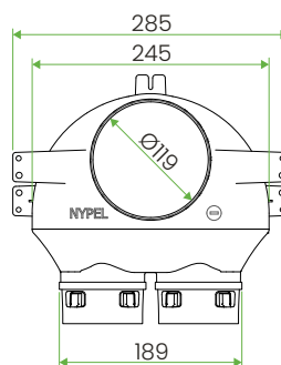
floor-mounted version
