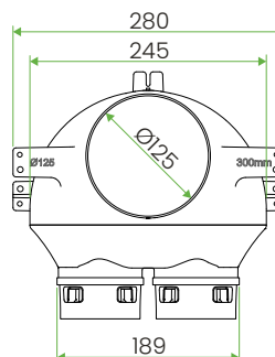
floor-mounted version
