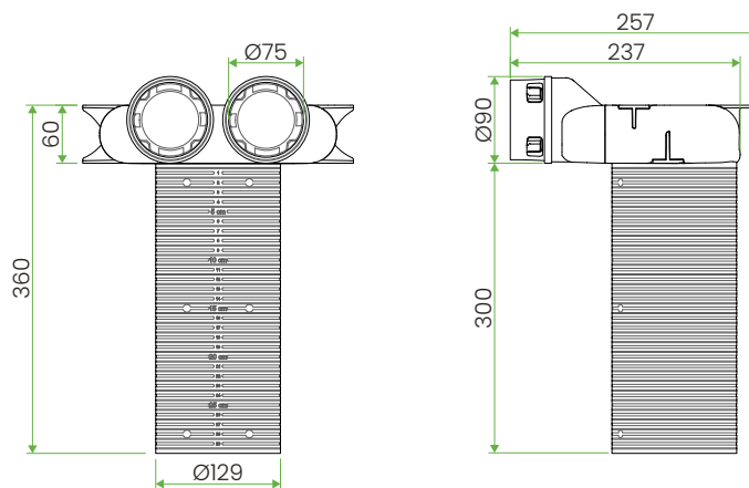
ceiling-mounted version
