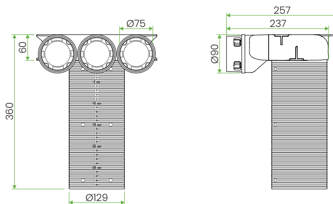
ceiling-mounted version
