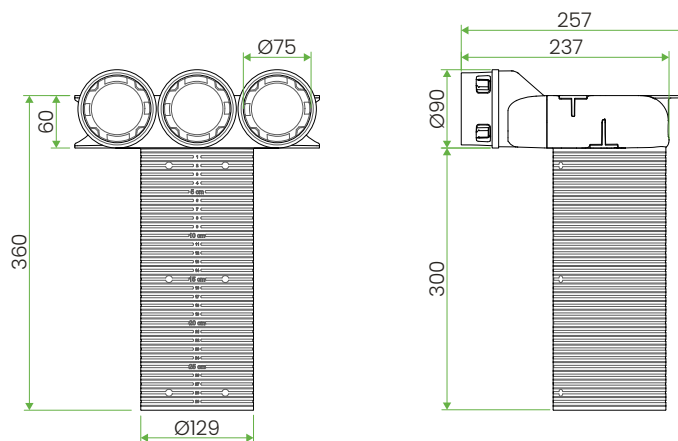
floor-mounted version
