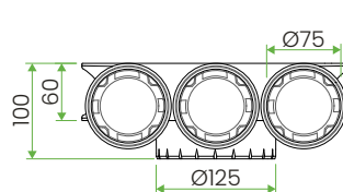
ceiling-mounted version
