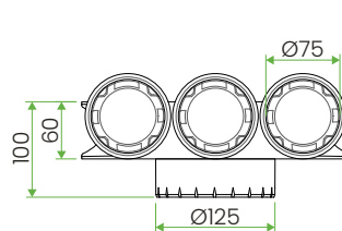
floor-mounted version
